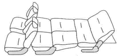
Second and third seats forming flat space (bed configuration 2)
